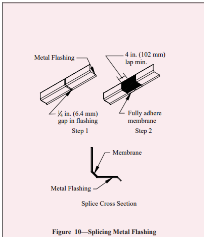
📷 Figure 10—Splicing Metal Flashing
