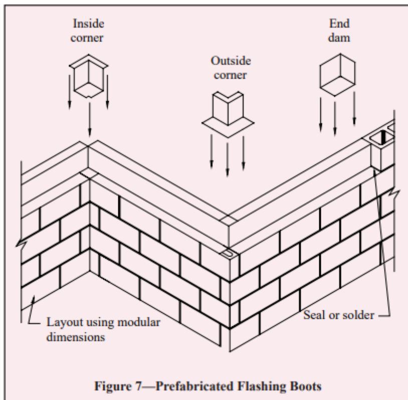
📷 Figure 7—Prefabricated Flashing Boots
