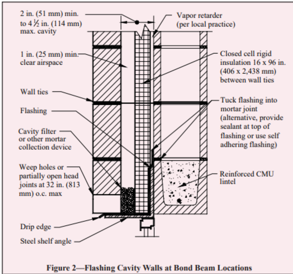
Figure 2—Flashing Cavity Walls at Bond Beam Locations
