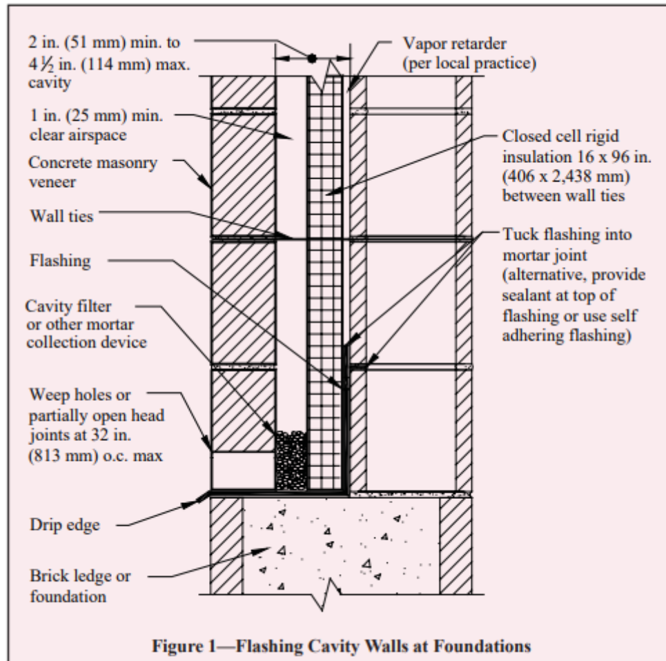
© Figure 1—Flashing Cavity Walls at Foundations
