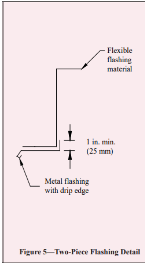
📷 Figure 5—Two-Piece Flashing Detail
