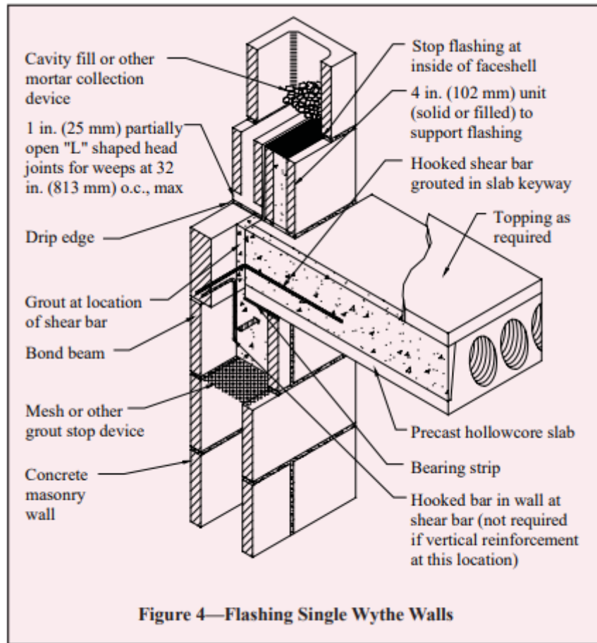
Figure 4—Flashing Single Wythe Walls
