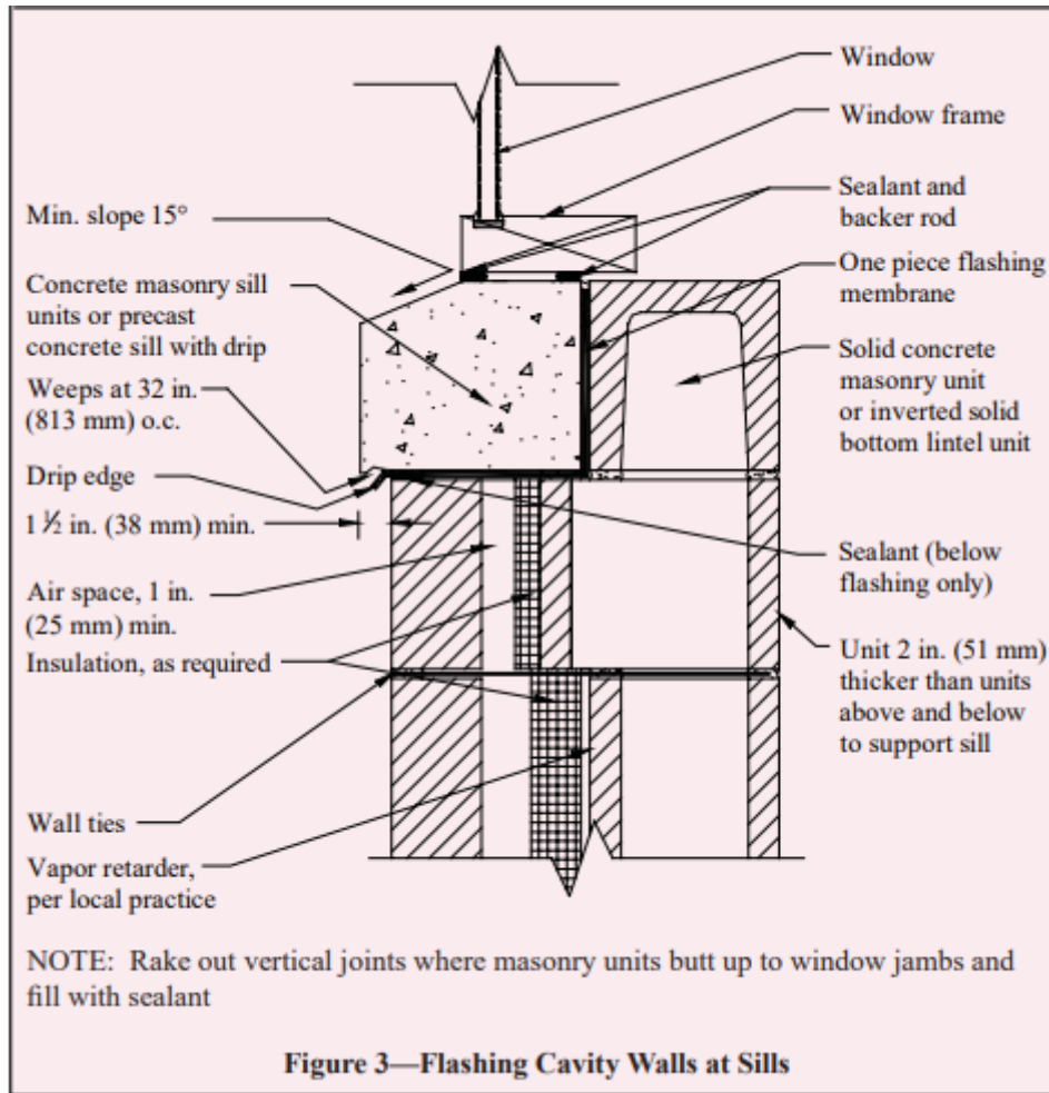
Figure 3—Flashing Cavity Walls at Sills
