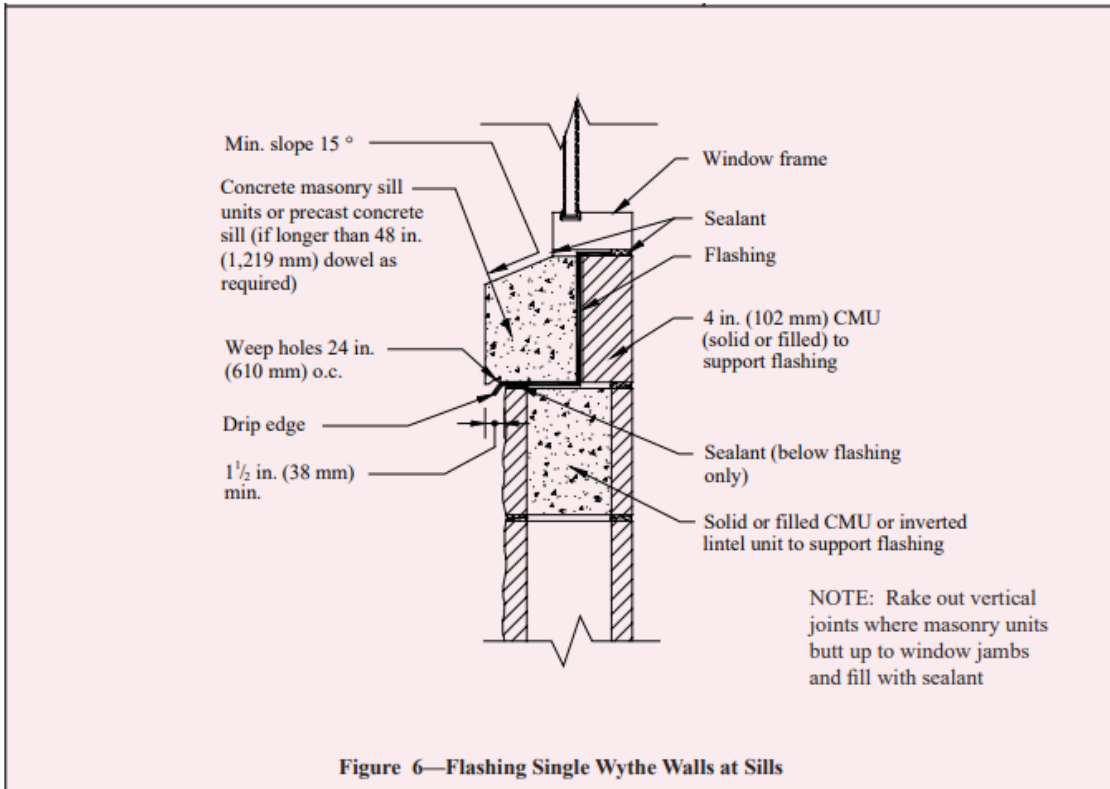
📷 Figure 6—Flashing Single Wythe Walls at Sills
