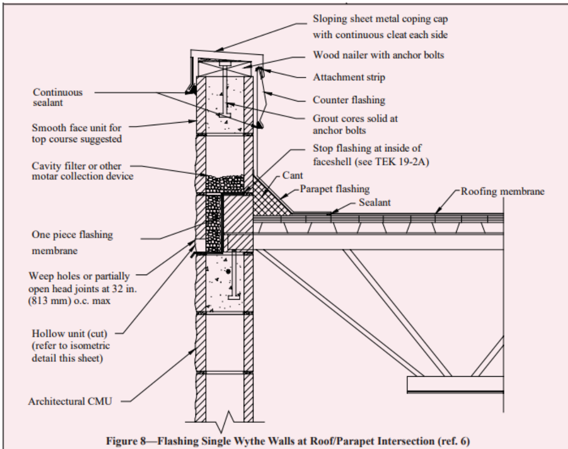
Figure 8—Flashing Single Wythe Walls at Roof/Parapet Intersection (ref. 6)
