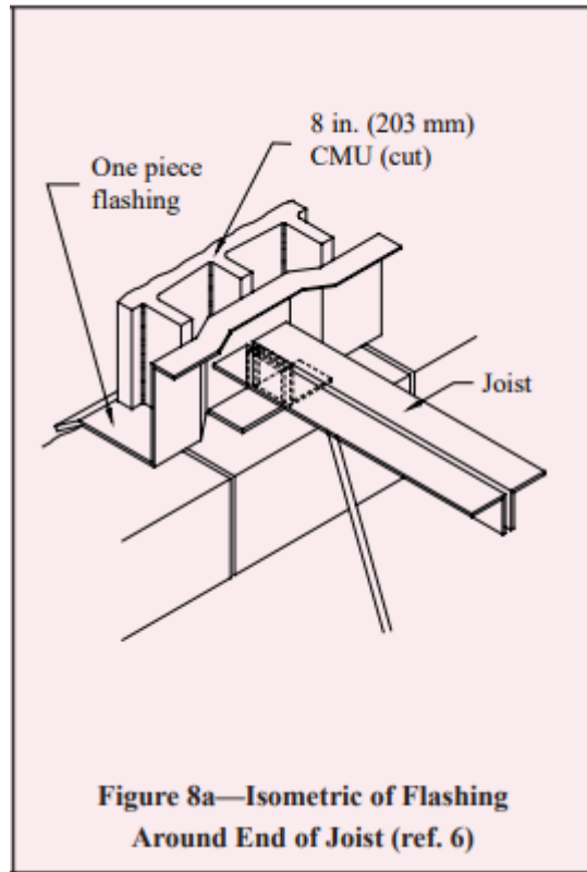
📷 Figure 8a—Isometric of Flashing Around End of Joist (ref. 6)
