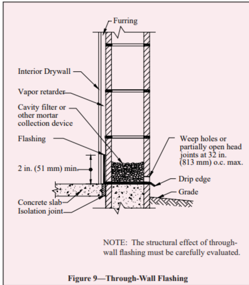
Figure 9—Through-Wall Flashing
