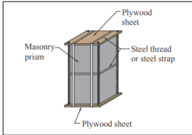
Figure 4-Transporting Prisms
