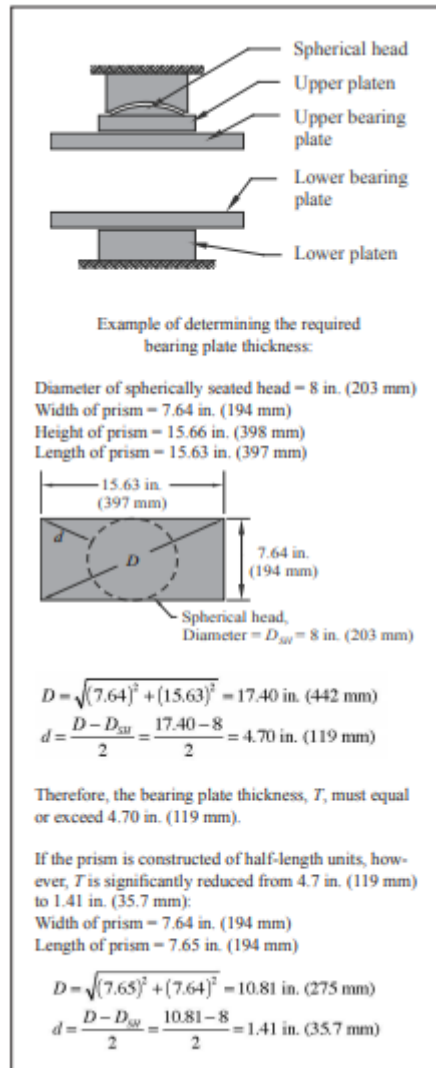
Figure 6—Determination of Bearing Plate Thickness
