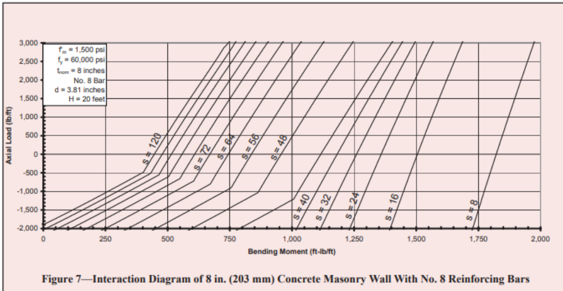
Figure 7—Interaction Diagram of 8 in. (203 mm) Concrete Masonry Wall With No. 8 Reinforcing Bars
