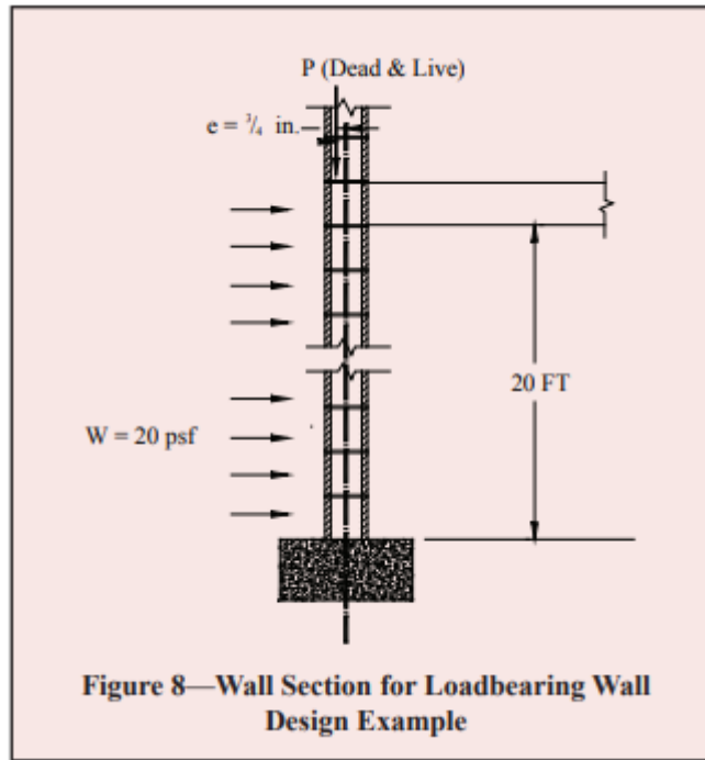
Figure 8—Wall Section for Loadbearing Wall Design Example
