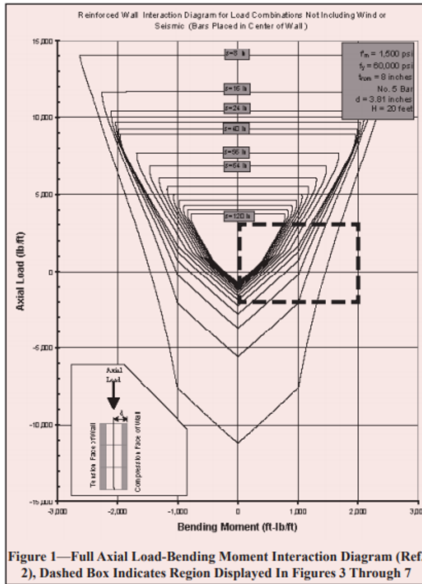
Figure 1—Full Axial Load-Bending Moment Interaction Diagram (Ref. 2), Dashed Box Indicates Region Displayed In Figures 3 Through 7
