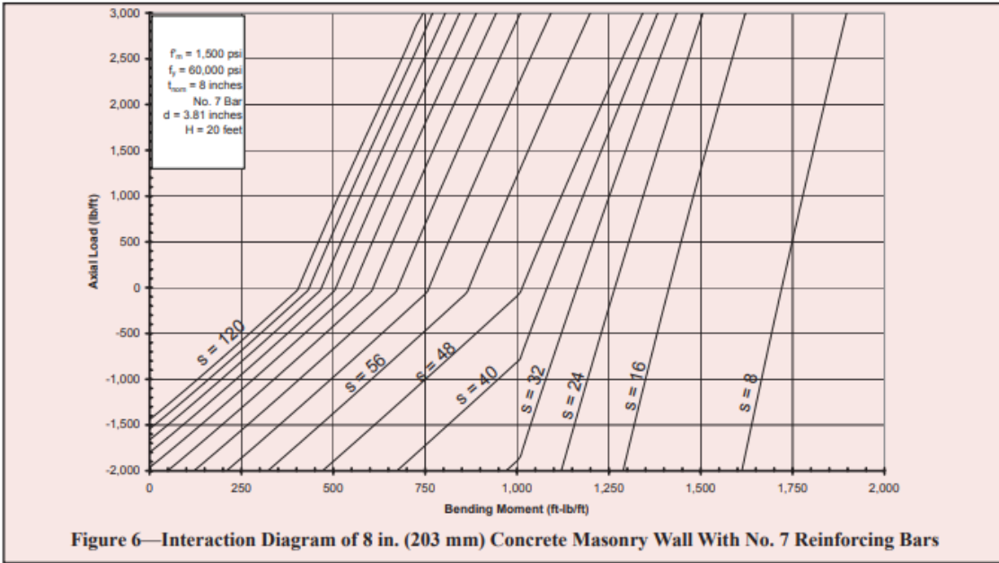
Figure 6—Interaction Diagram of 8 in. (203 mm) Concrete Masonry Wall With No. 7 Reinforcing Bars
