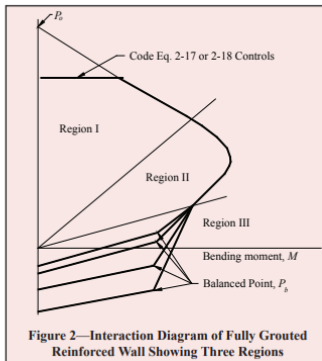
Figure 2—Interaction Diagram of Fully Grouted Reinforced Wall Showing Three Regions
