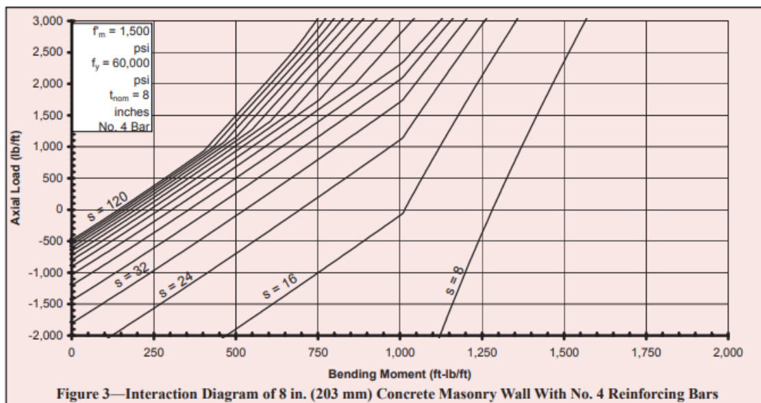
Figure 3—Interaction Diagram of 8 in. (203 mm) Concrete Masonry Wall With No. 4 Reinforcing Bars
