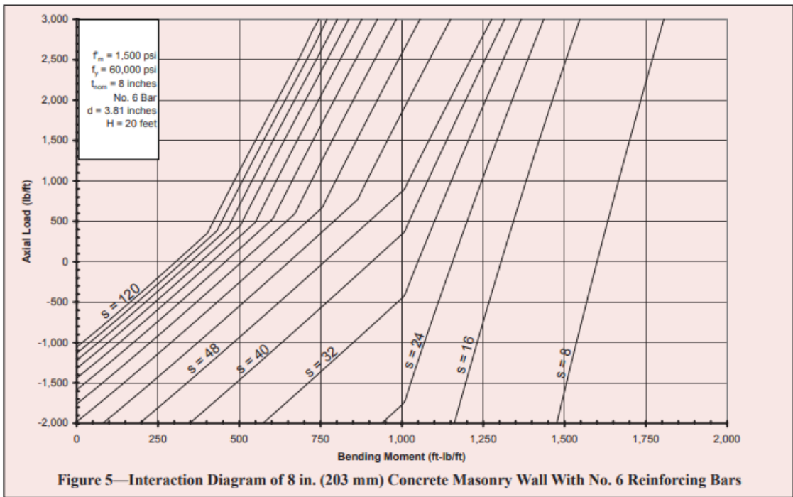
Figure 5—Interaction Diagram of 8 in. (203 mm) Concrete Masonry Wall With No. 6 Reinforcing Bars
