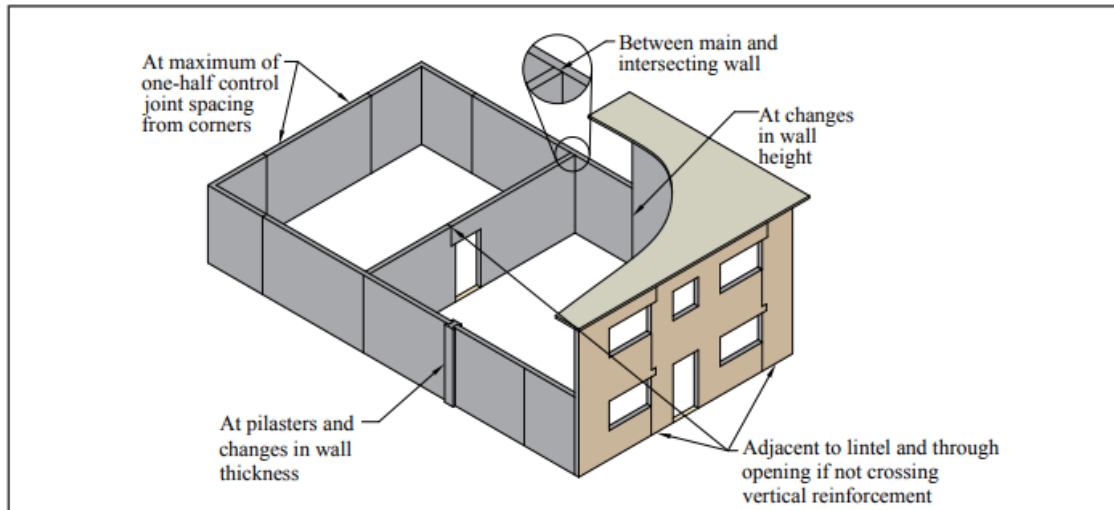
📷 Figure 1a—Typical Control Joint Locations for Unreinforced Masonry
