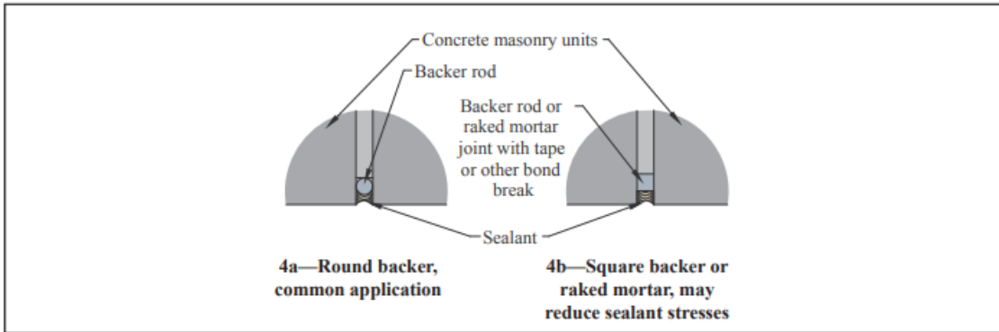
📷 Figure 4—Detail of Control Joint Surface (ref. 6)
