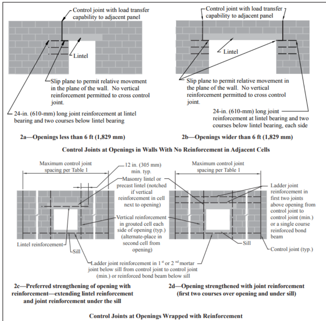
Figure 2—Control Joints at Openings
