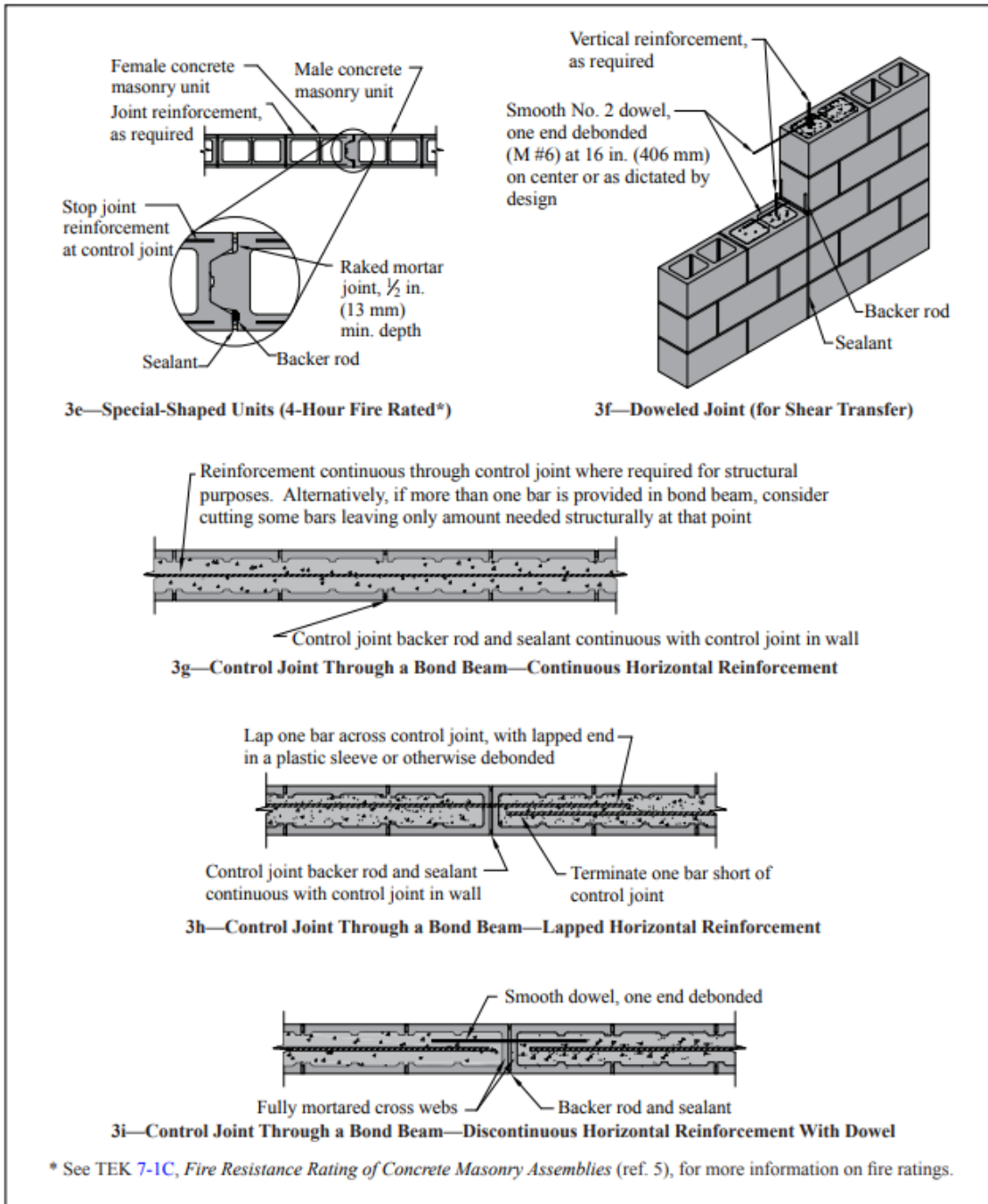
Figure 3—Typical Control Joint Details
