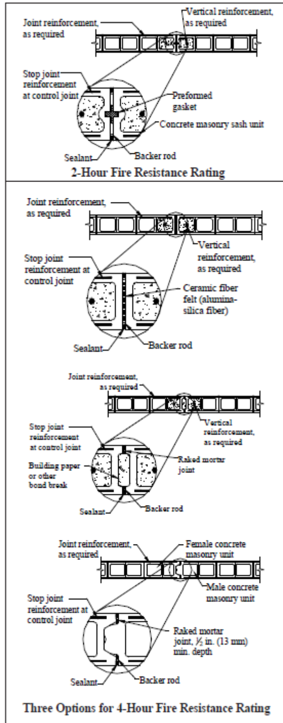
Figure 3—Control Joints for Fire Resistant Concrete Masonry Assemblies (ref. 1)
