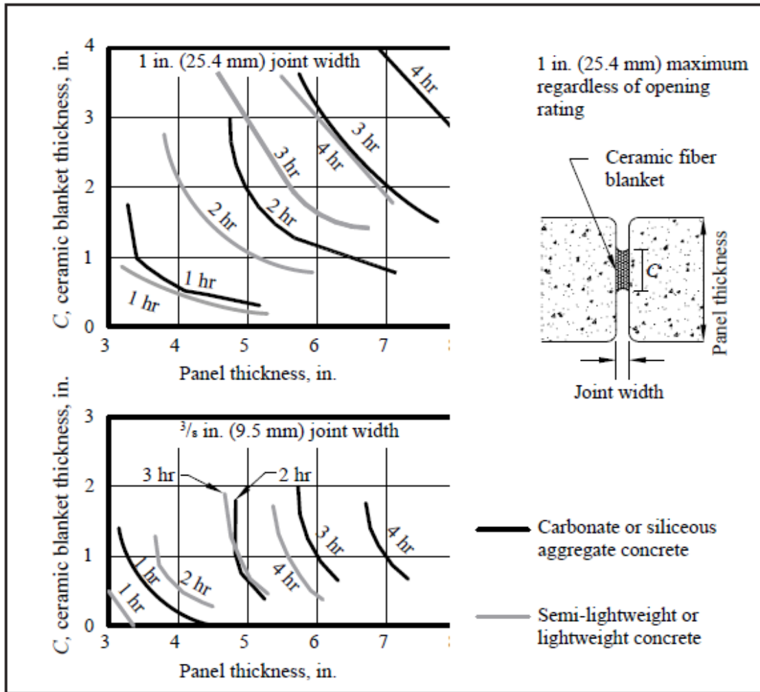
Figure 4—Ceramic Fiber Joint Protection
