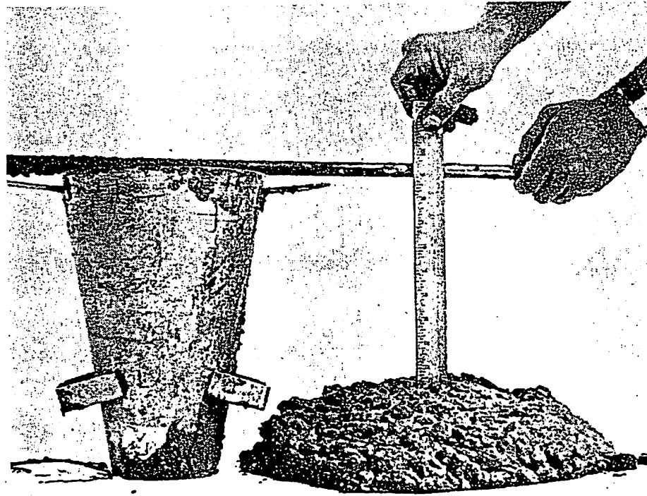
Fig. 14-2. Slump test for consistency of concrete. Figure A illustrates a low slump, Figure B a high slump.
